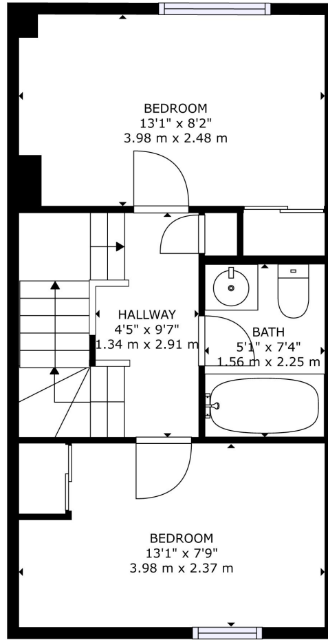
FLOOR 3
