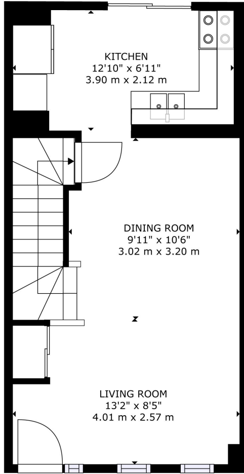
FLOOR 2
